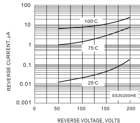
Fig.6- TYPICAL REVERSE CHARACTERISTICS
