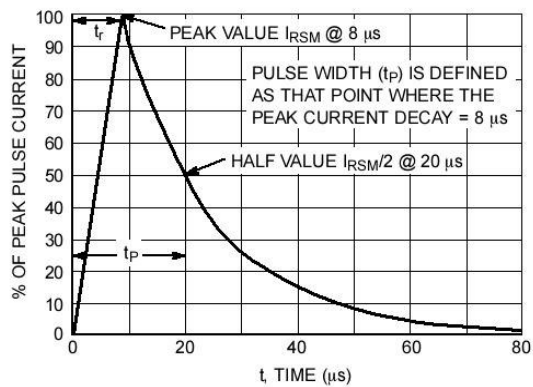
Fig.5 8/20µS Peak Pulse Current Waveform
