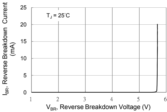
Fig.1 Typical Reverse Characteristics
