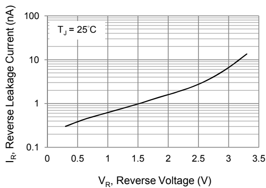
Fig.3 Reverse Leakage Current
