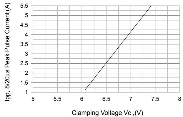
Fig.4 Typical Peak Clamping Voltage
