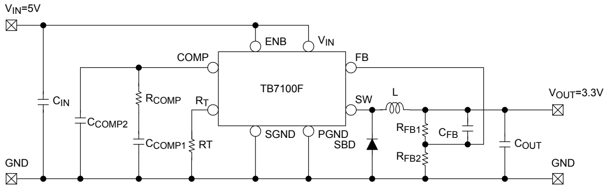
Figure 1: TB7100F application circuit example
