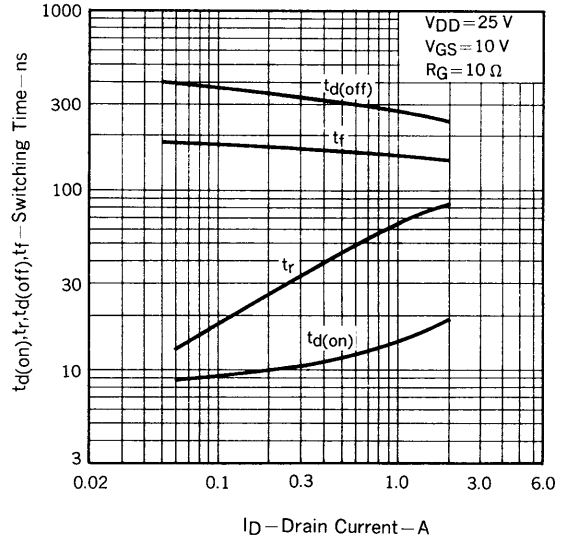
SWITCHING CHARACTERISTICS
