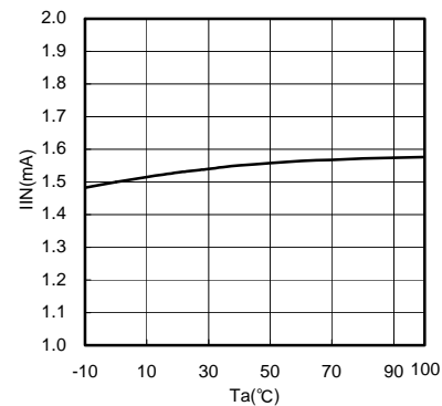
Fig.30 Ta-IIN
