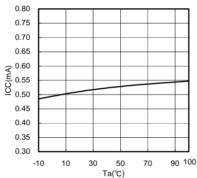
Fig.28 Ta-ICC
