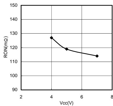
Fig.36 VCC-RON
