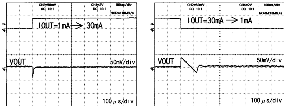
Fig.14 Load Transient response ( C_o=2.2 \mu F )
