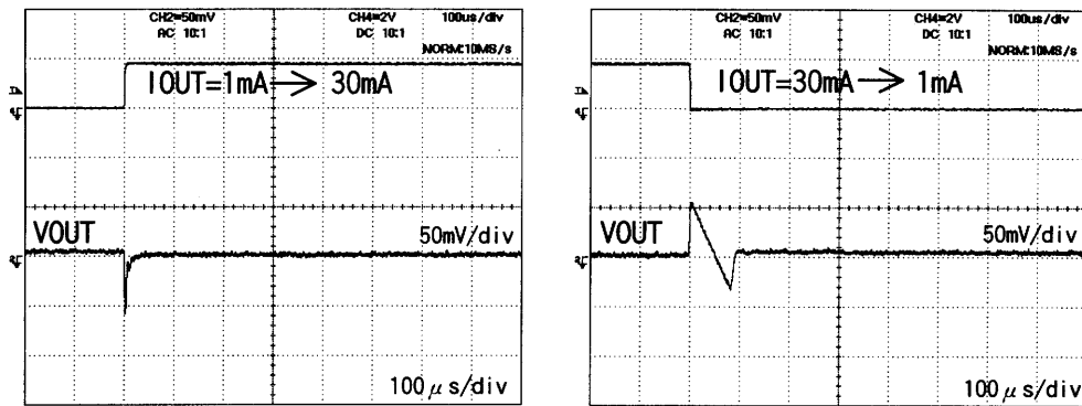
Fig.13 Load Transient response ( C_o=1.0 \mu F )
