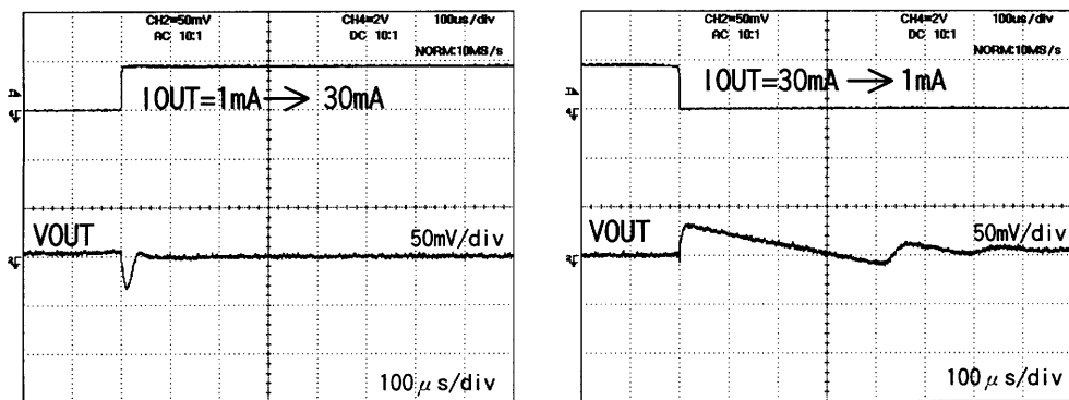
Fig.15 Load Transient response ( C_o=10 \mu F )
