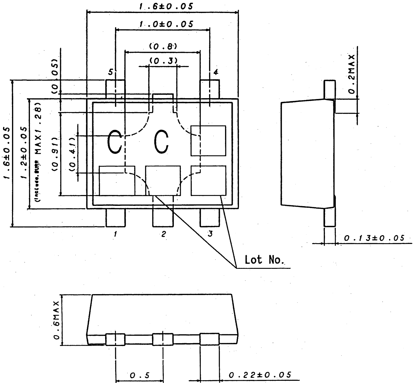
Fig.1 PACKAGE (Plastic Mold) (Unit:mm)
