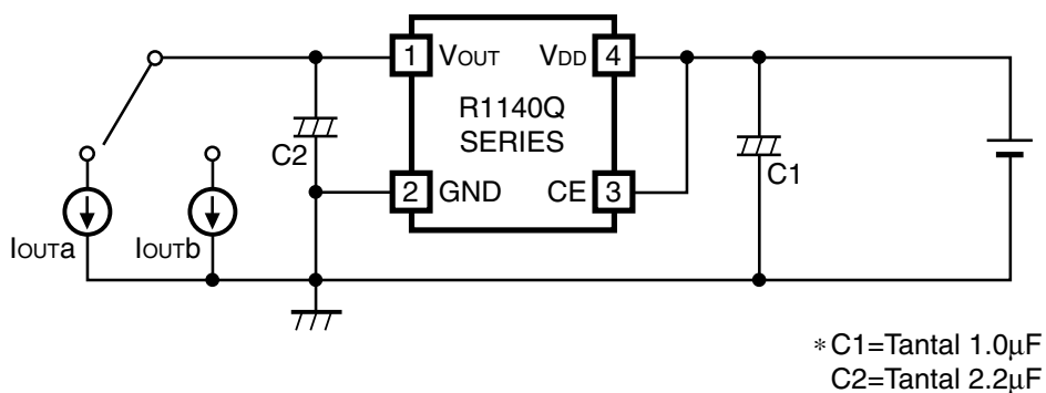
Fig.4 Load Transient Response Test Circuit
