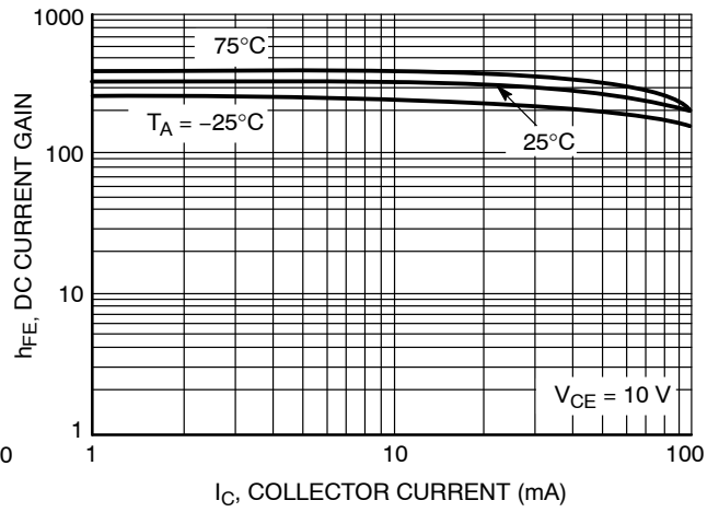
Figure 58. DC Current Gain
