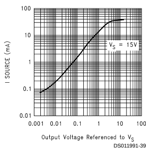
Sourcing Current vs Output Voltage (15V)
