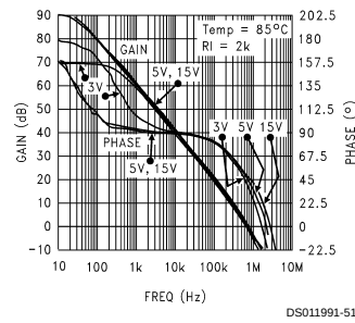
Open Loop Frequency Response @ 85^\circ C
