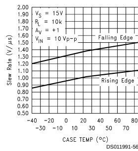
Slew Rate vs Temperature
