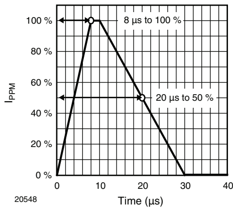
20548 Fig. 2 - 8/20 \mu\text{s} Peak Pulse Current Wave Form acc. IEC 61000-4-5
