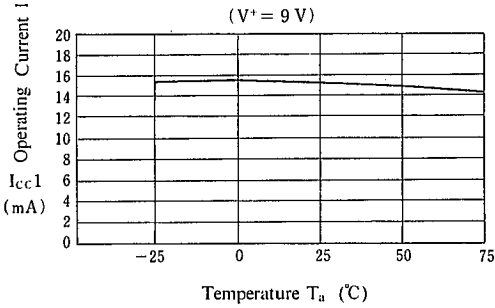
Operating Current 1 vs. Temperature ( V^+ = 9\text{ V} )
