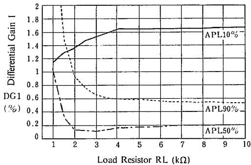
Differential Gain 1 vs. Load Resistor ( T_a=25^\circ\text{C} )
