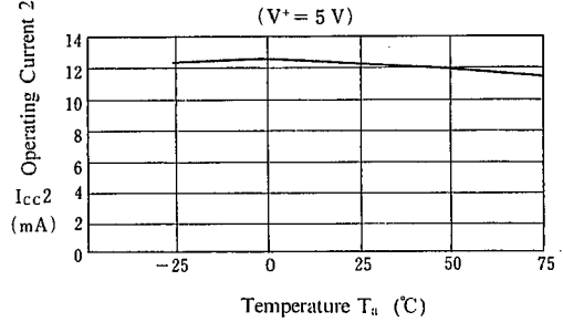
Operating Current 2 vs. Temperature ( V^+ = 5\text{ V} )
