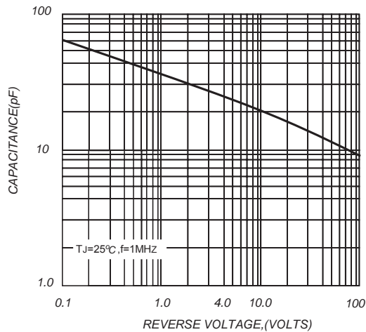
FIG.3-TYPICAL JUNCTION CAPACITANCE
