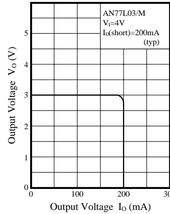
Over-current Limiting Characteristics V_O - I_O
