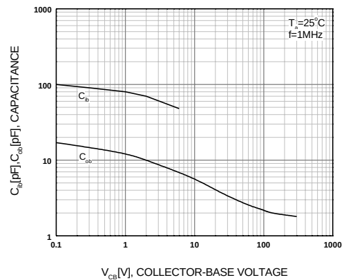
Figure 4. Capacitance
