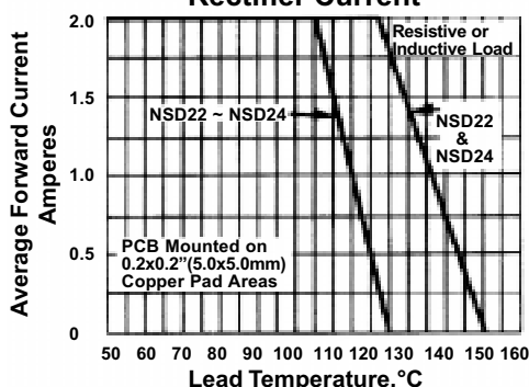
Fig.1 - Derated Curve for Output Rectifier Current
