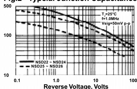
Fig.2 - Typical Junction Capacitance
