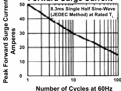
Fig.4 - Maximum Non-Repetitive Peak Forward Surge Current
