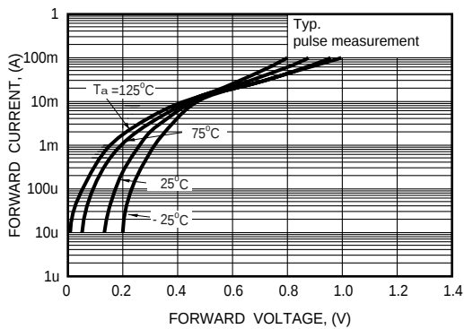
FIG. 1 - FORWARD CHARACTERISITICS
