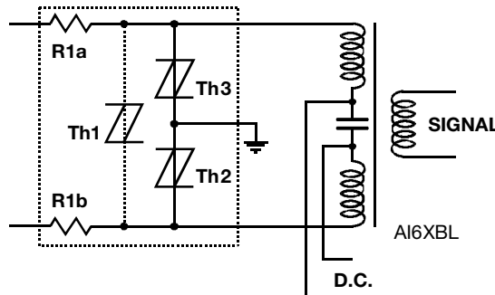
Figure 17. ISDN Protection
