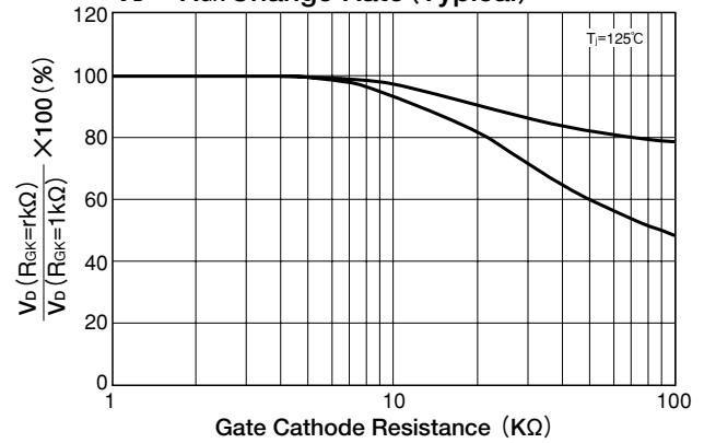
V_D - R_{GK} Change Rate (Typical)
