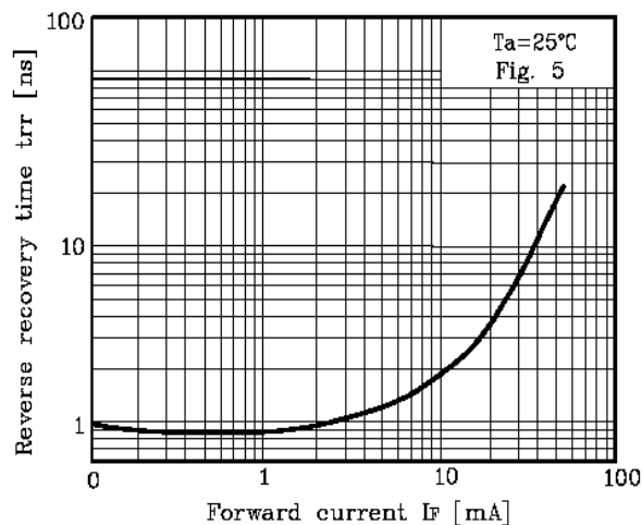
Fig 4. t_{rr} - I_F
