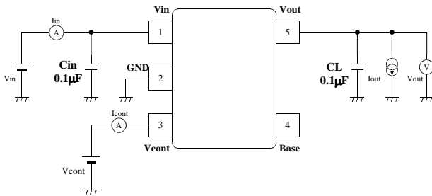
Standard circuit (Iout 100mA)
