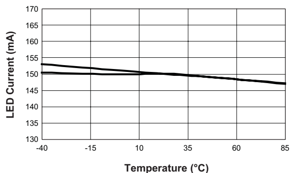
Flash Current Matching vs. Temperature (150mA/Ch; Data 6)
