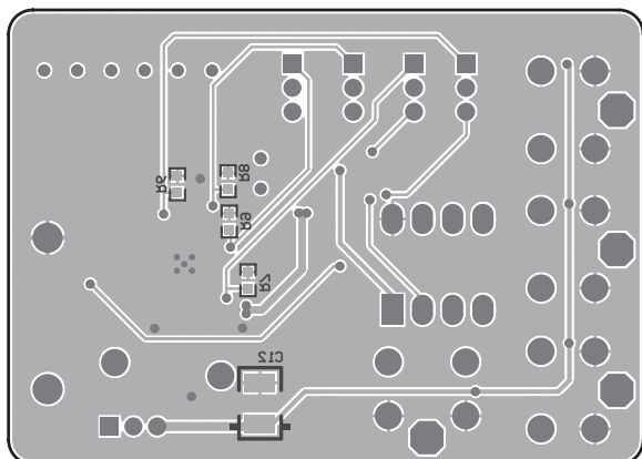
Figure 5: Example PCB Layout.
