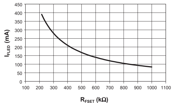
Figure 4: Maximum Flash LED Current vs. R_{\text{FSET}}
