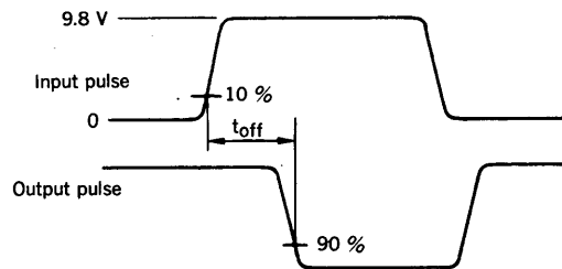
t_{off} Voltage Waveforms ( V_{BB} = -8.0\text{ V} )
