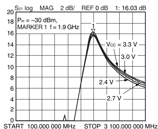
S 21 -FREQUENCY
