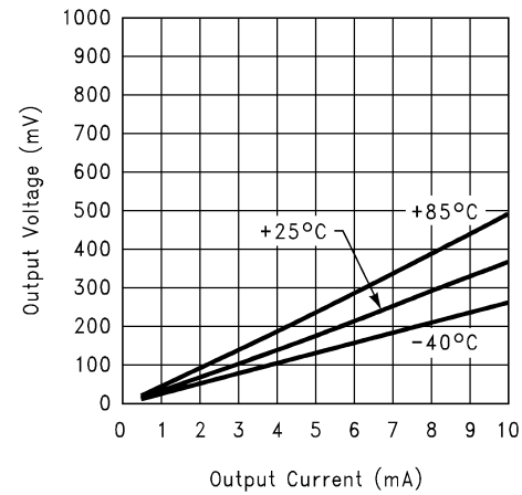
Output Sinking Current vs. Output Voltage @ 5V
