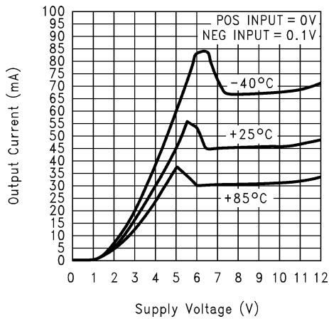
Output Sinking Current vs. Supply Voltage
