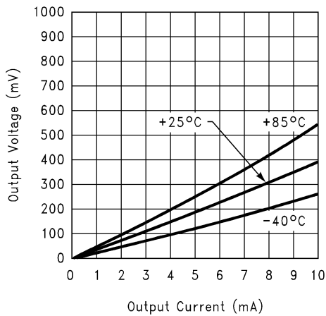
Output Sinking Current vs. Output Voltage @ 15V
