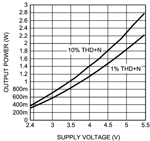
Output Power vs Supply Voltage R_L = 4\Omega
