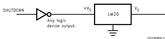
FIGURE 7. Conserving Power Dissipation with Shutdown
