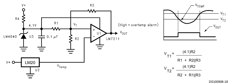
FIGURE 6. Centigrade Thermostat
