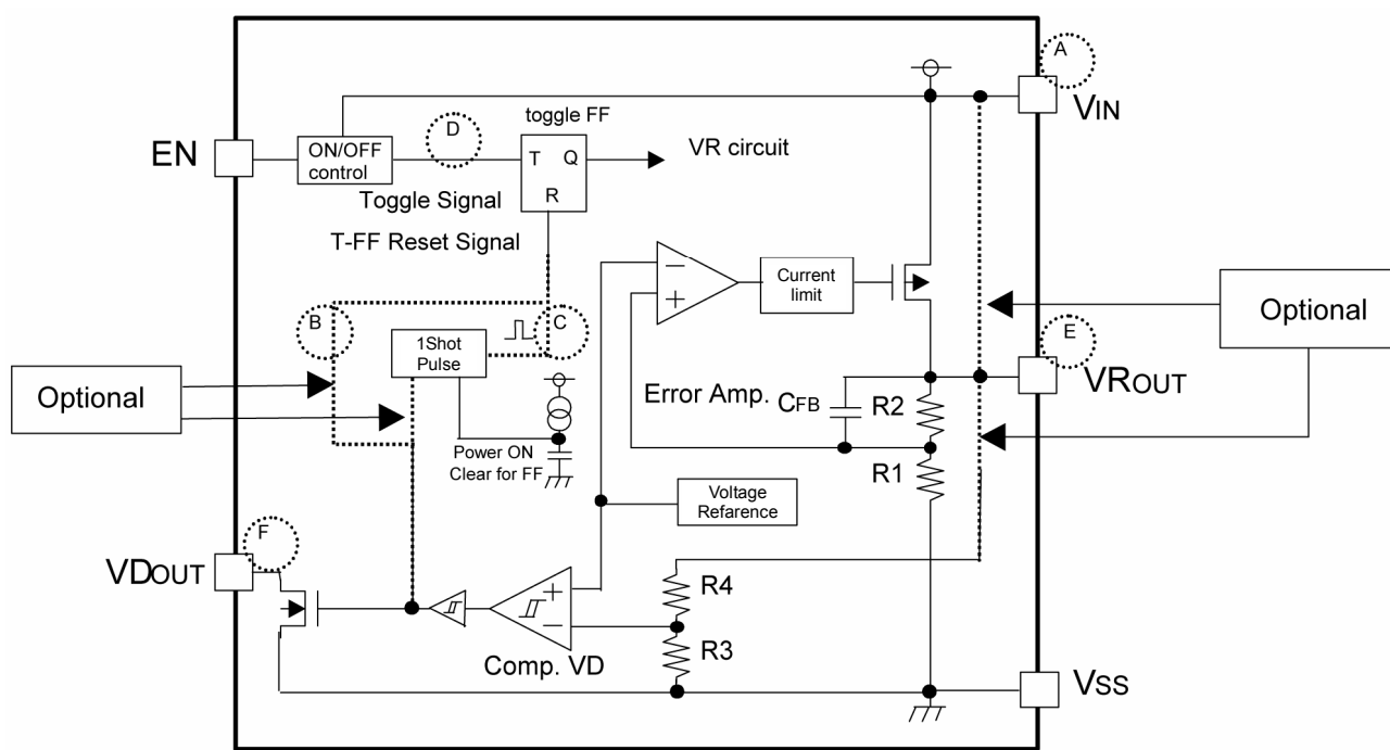
Block Diagram for XC6405B Series Timing Chart
