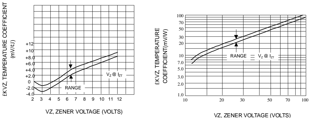
Fig. 2-TEMPERATURE COEFFICIENTS
