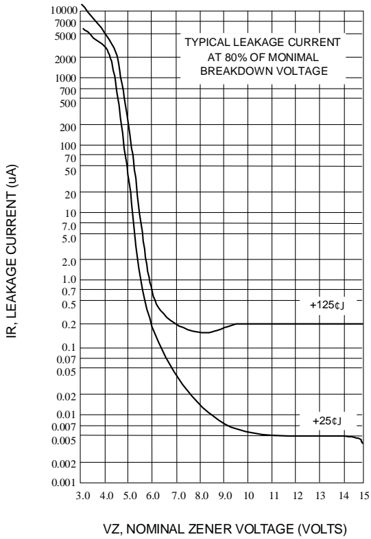
Fig. 8-TYPICAL LEAKAGE CURRENT
